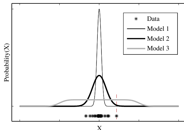
Fig. 2. Model complexity and evidence. See text for details.
