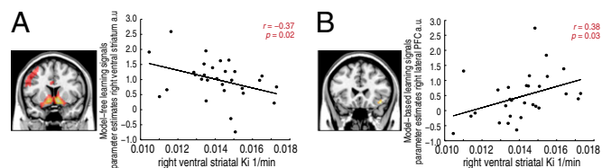
Fig. 3. Presynaptic dopamine and neural learning signatures. Correlation between right ventral striatal presynaptic dopamine K_i and (A) model-free learning signals in right ventral striatum ( r = -0.37 ; P = 0.02 ) and (B) model-based signatures in right lateral prefrontal cortex ( r = 0.38 ; P = 0.03 ).
